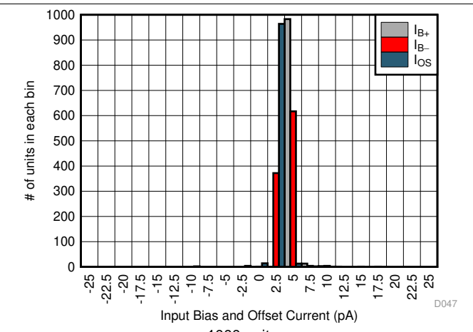
Figure 34. Input Bias and Offset Current Histogram
