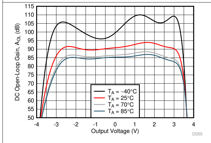
Figure 23. DC Open-Loop Gain vs Output Voltage
